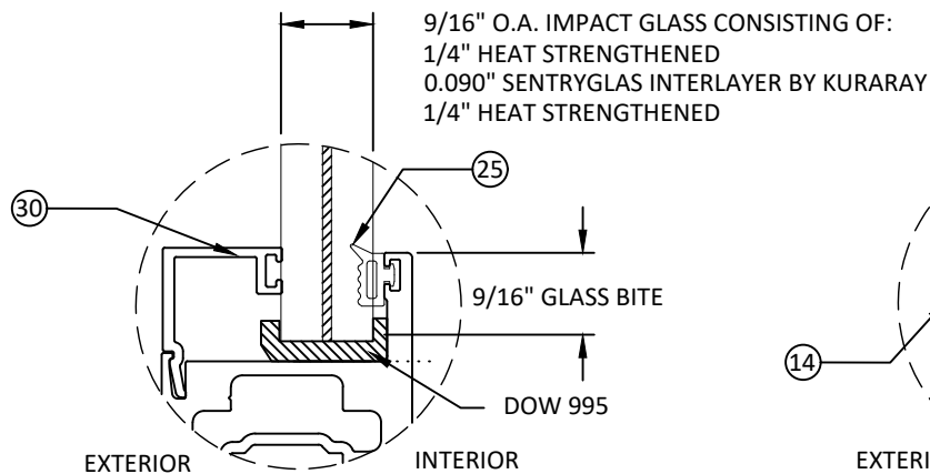
GLAZING DETAIL 1
