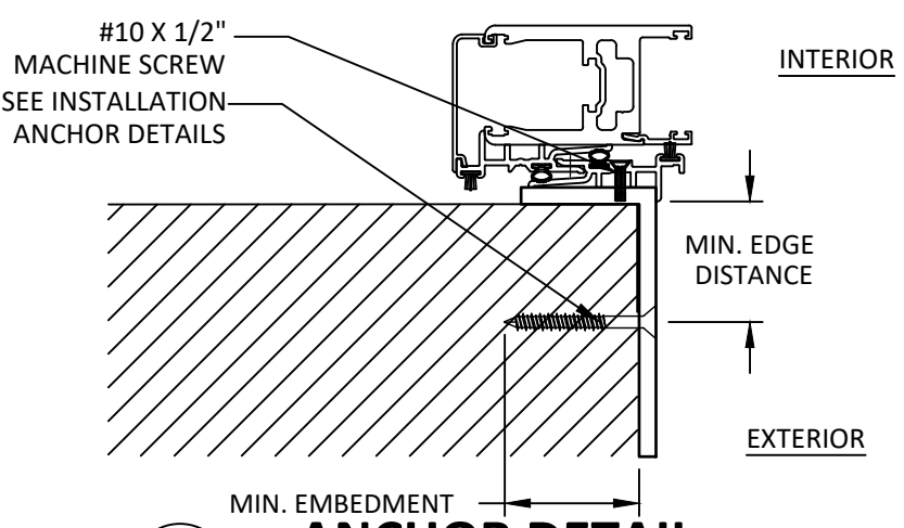
C 9 ANCHOR DETAIL INSIDE POCKET BRACKET INSTALLATION
