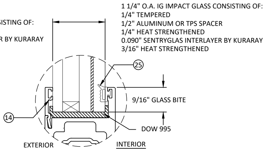
GLAZING DETAIL 2
