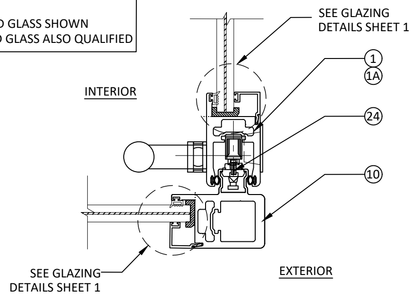
B 6 HORIZONTAL SECTION OUTSIDE CORNER DETAIL
